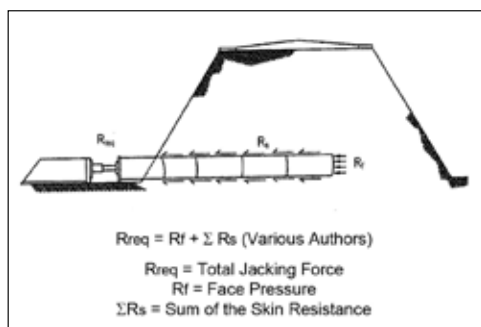
Figure 1: Free Body Diagram of the Forces acting on Pipe Jacking methods
