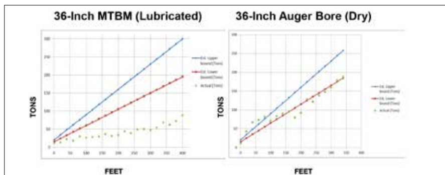
Figure 2: Axial loading development graphs of similar MTBM and Auger Boring installations in similar ground.
